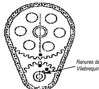
Figure 6 Normal
