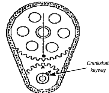
Figure 7 4° Advance
