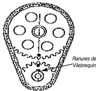
Figure 3 Normal
