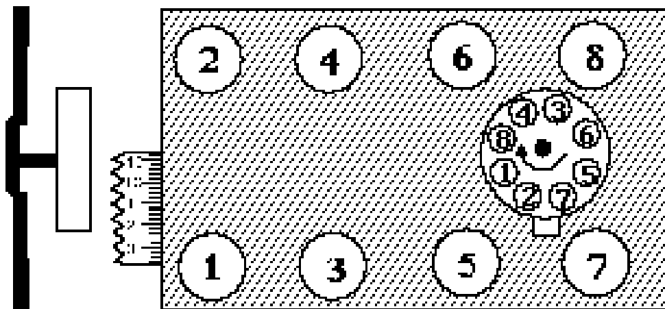
Figure 1- Chevrolet 262-400 c.i.d. V8
